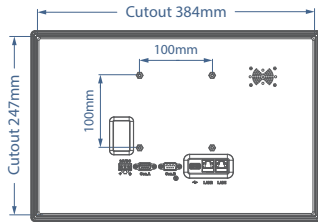
Rear View
