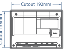
Rear View
